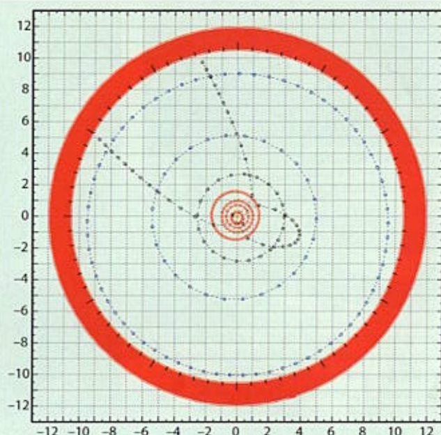
7: The orbits of the six classical planets, two comets (1P/Halley and 2P/Encke) and the main-belt asteroid 1 Ceres. Tiles are placed on the ground at 16-day intervals for the terrestrial planets (Mercury, Venus, Earth and Mars), at 80-day intervals for Ceres and the comets, and 160-day intervals for Jupiter and Saturn.
